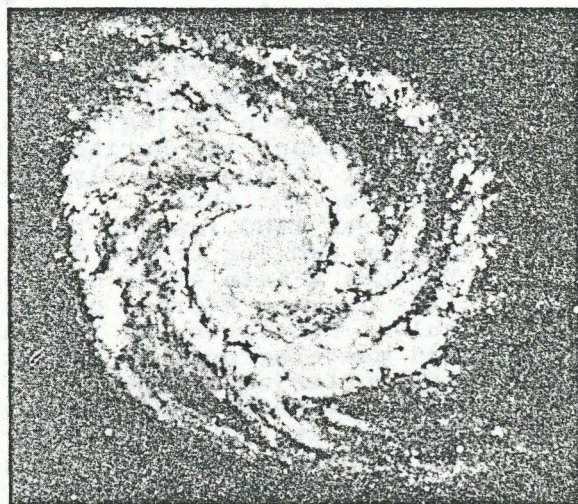
Whirlpool galaxy (M51)
